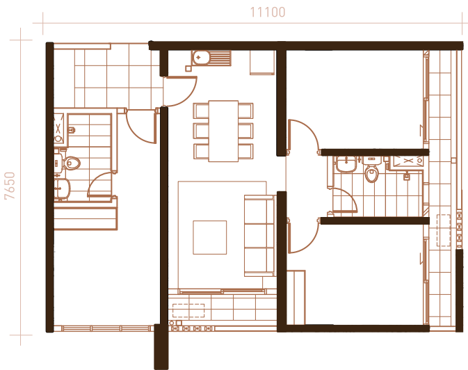
TYPE B2 - 914 sq ft
